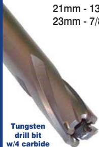
Drills out female/male threads on lug nut/stud only!
